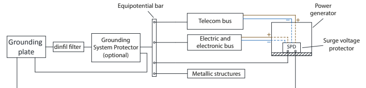
Figure 5. General diagram of protection in a boat.
