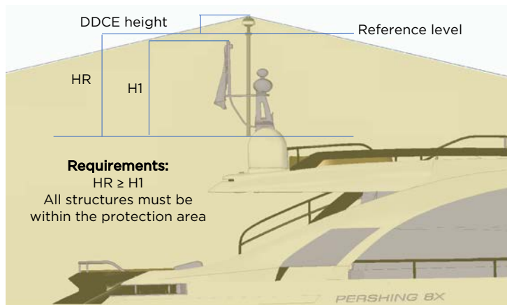
Figure 7. Height requirements for the DDCE in respect with the rest of the installed elements.
