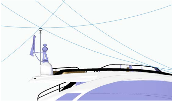
Figure 3. Detail of the Rolling Spheres Method in the upper area of the mast of the boat in figure 2.
