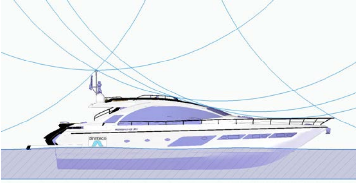
Figure 2. SPCR Rolling Spheres Method Level I of Protection (R = 66 ft) in a medium boat.
