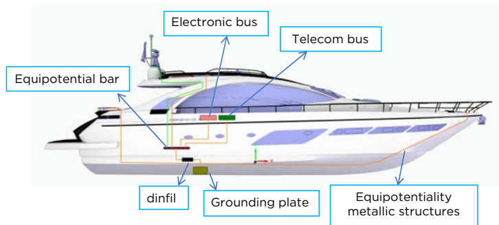
Figure 4. General detail of equipotential system.
